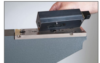
Pre-aligned lower tool holders.
