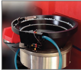
Modular Autofeed System.
