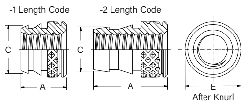
Diamond Knurl Thread sizes 0-80, 2-56 and M2
