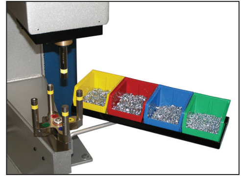
Optional QX4™ manual tooling.
